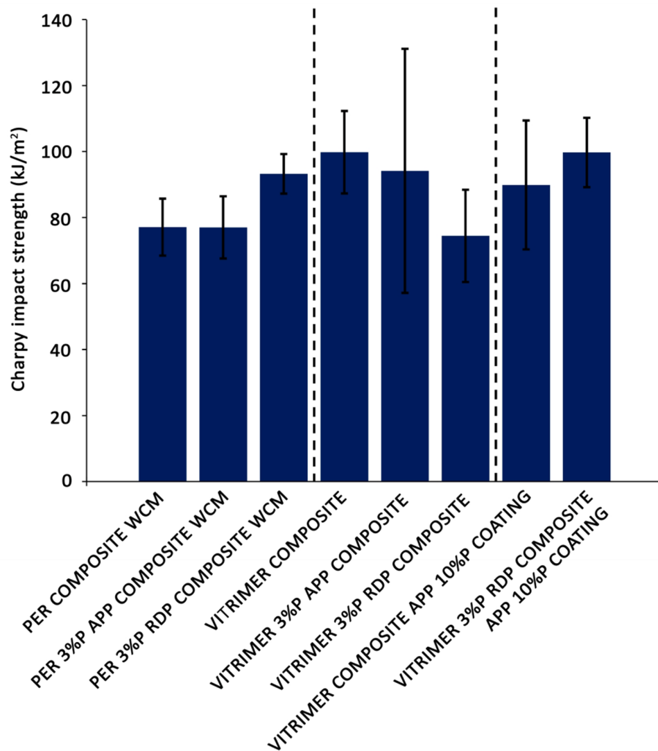
Fig. 10. Charpy impact test results of the reference and flame retarded vitrimer composites without and with intumescent coating compared to PER epoxy resin benchmark composite.
