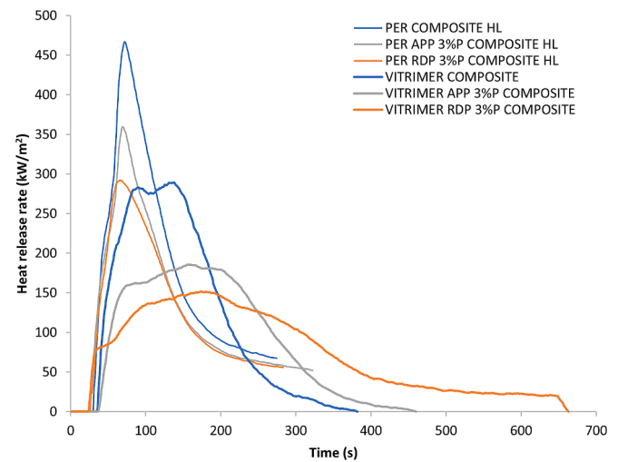
Fig. 2. The heat release rate of reference and flame retarded vitrimer and hand-laminated (HL) epoxy resin composites.
