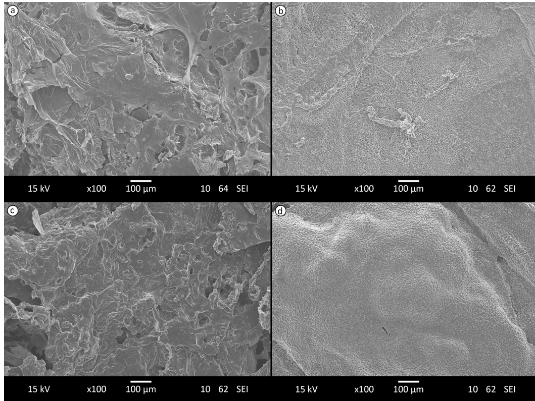
Fig. 7. Typical SEM images of the combustion residues (a) inner and (b) outer layers of the coated reference vitrimer composite (VITRIMER COMPOSITE APP 10 %P COATING), (c) inner and (d) outer layers of the coated vitrimer composite flame retarded with RDP (VITRIMER RDP 3 %P COMPOSITE APP 10 %P COATING).
