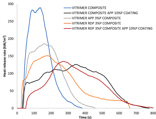
Fig. 5. The heat release rate of reference and flame retarded vitrimer composites without and with intumescent coating.
