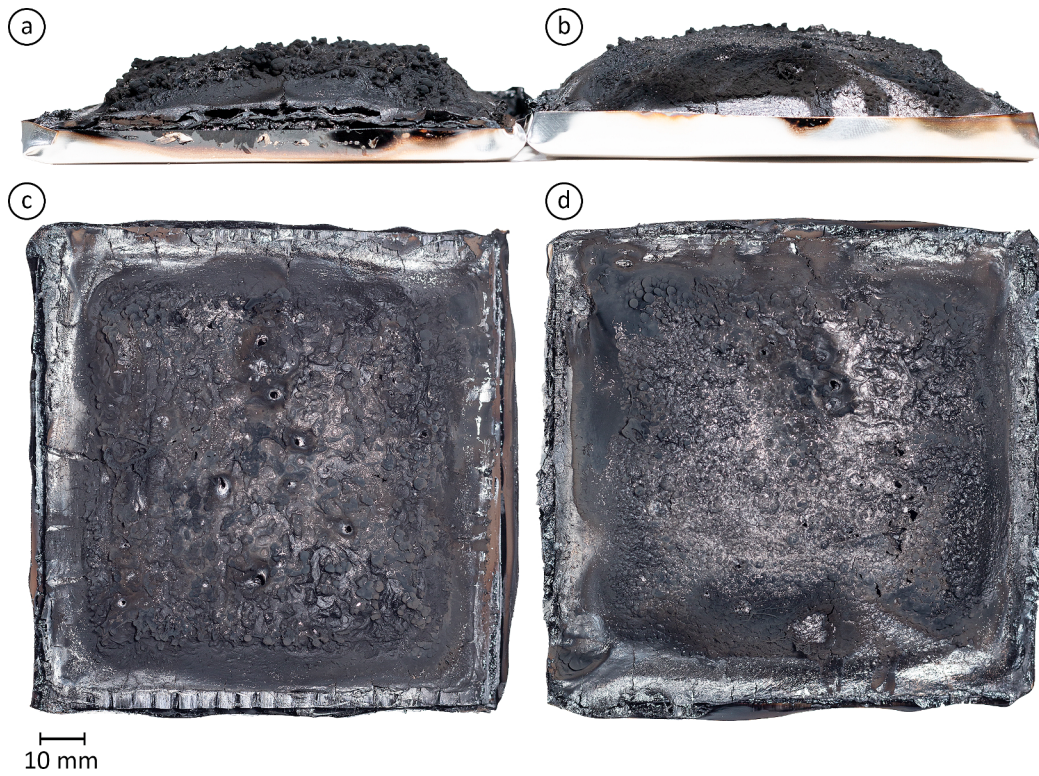
Fig. 6. The residue of composites with intumescent coating: (a) front view of VITRIMER COMPOSITE APP 10 %P COATING, (b) front view of VITRIMER RDP 3 %P COMPOSITE APP 10 %P COATING, (c) top view of VITRIMER COMPOSITE APP 10 %P COATING, (d) top view of VITRIMER RDP 3 %P COMPOSITE APP 10 %P COATING.
