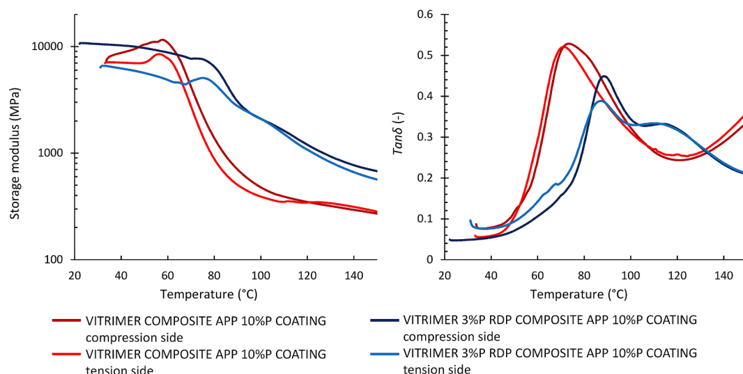
Fig. 9. Storage modulus and \tan\delta graphs of the reference and RDP flame retarded vitrimer composites with intumescent coating.
