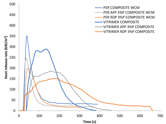
Fig. 3. The heat release rate of reference and flame retarded vitrimer and wet-compressed (WCM) epoxy resin composites.
