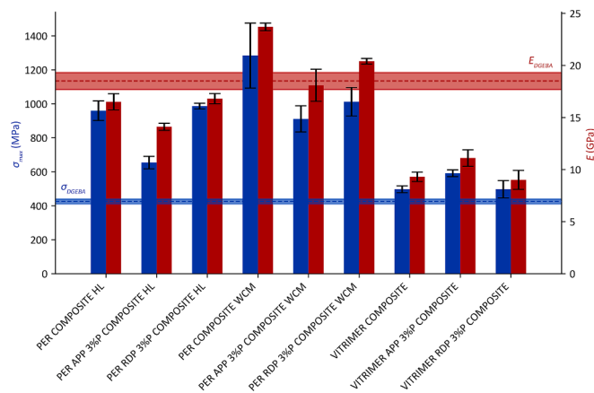
Fig. 4. Tensile test results of reference and flame retarded epoxy resin and vitrimer composites compared to benchmark DGEBA hand-laminated composite [31].
