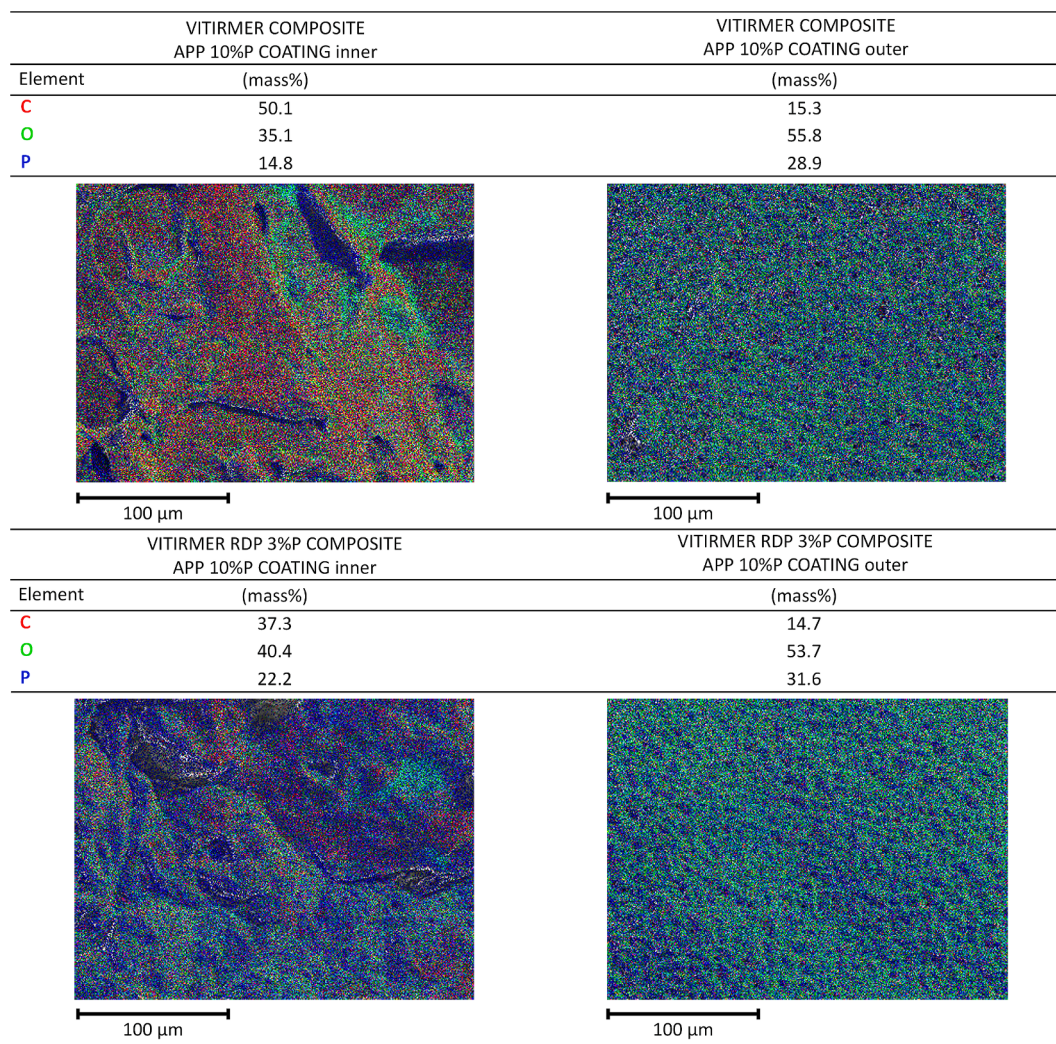
Fig. 8. Elemental composition of the inner and outer part of the mass loss type cone calorimetry residues of coated vitrimer composites by SEM-EDS (colour coding of elemental maps: carbon – red, oxygen – green, phosphorus – blue.).
