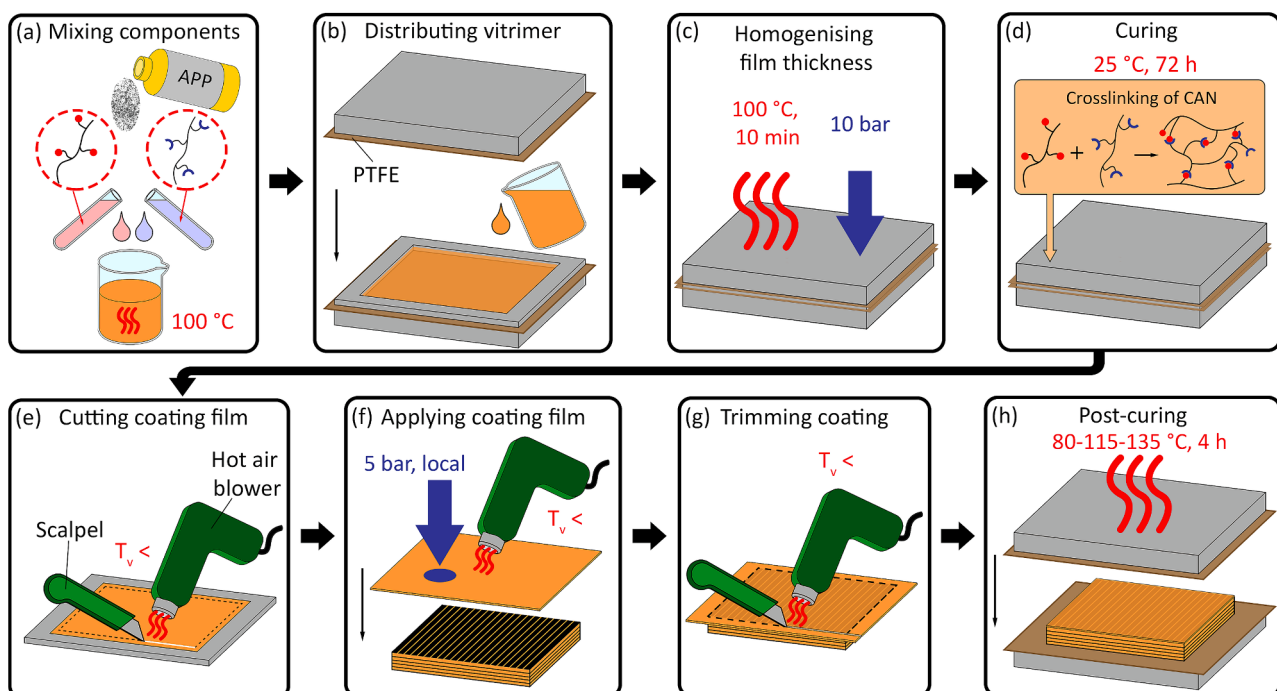
Fig. 1. Preparation of vitrimer-based flame retardant coatings and their application onto the composite.
