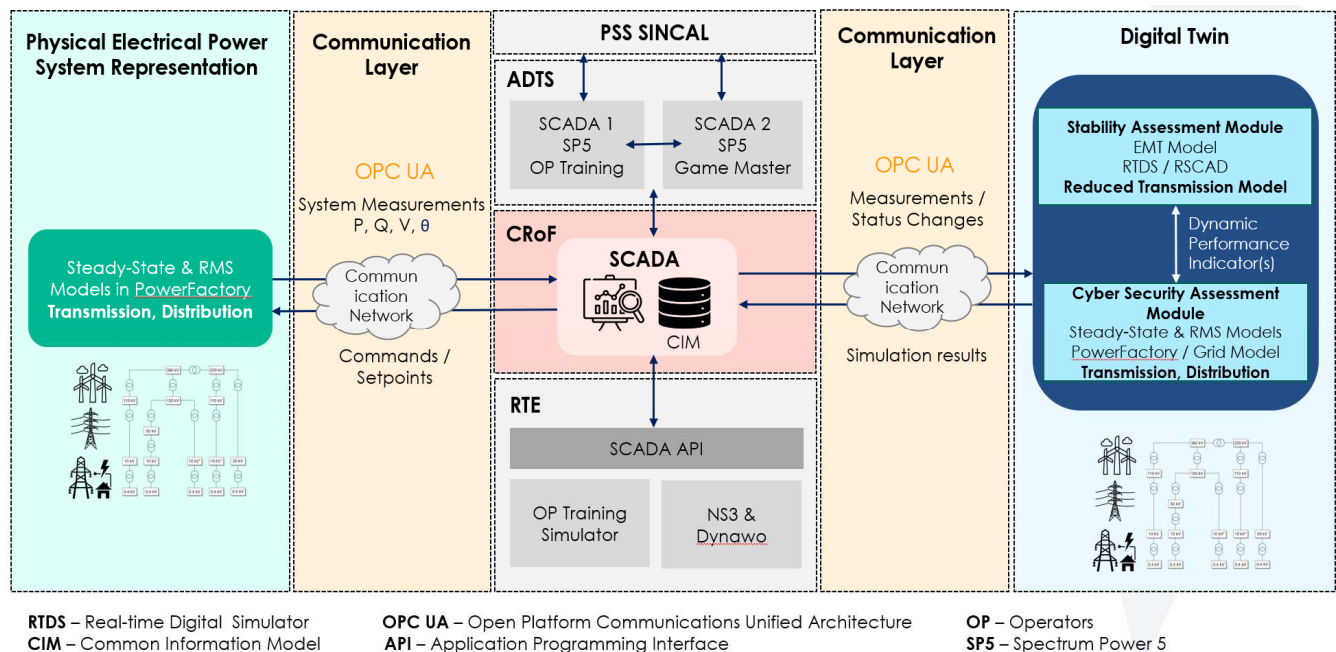
Fig. 4. The Dutch integrated digital twin architecture ([4])
