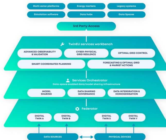
Fig. 2. TwinEU architecture ([3])
