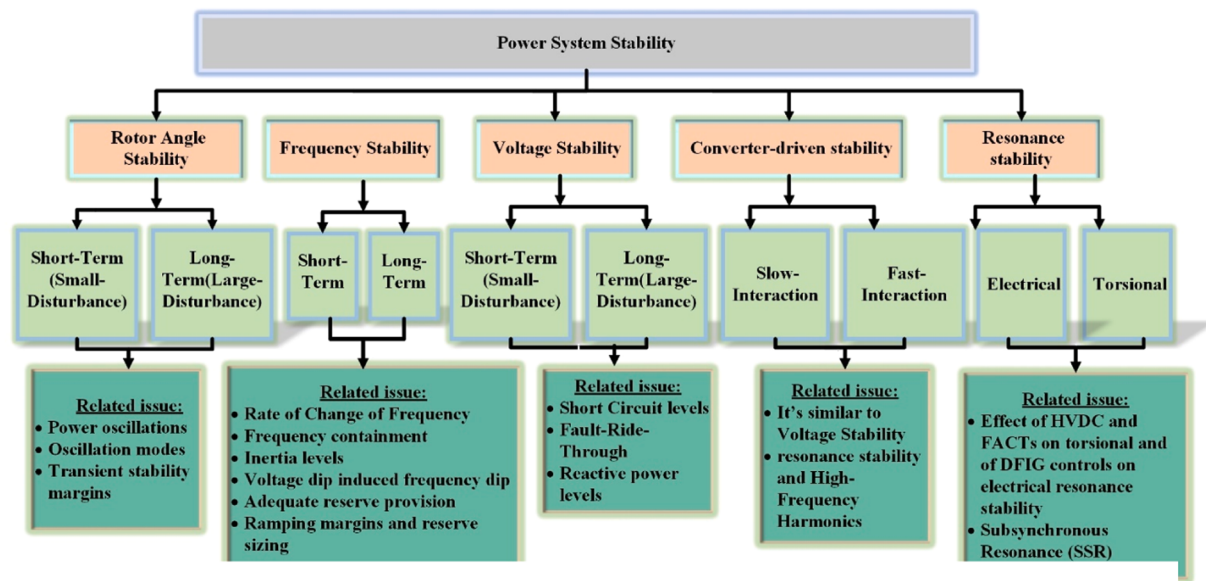
Fig. 7. Power system stability classification.
