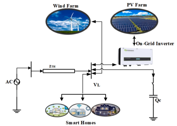
Fig. 9. Single line diagram of integration of RESs and capacitor bank.
