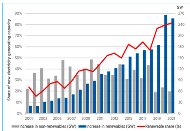
Fig. 2. Annual Power Capacity Growth of Renewable Energy (Anderson and Fouad, 2008).
