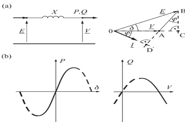
Fig. 8. A simplified representation circuit: (a) circuit and phasor diagram, (b) Active power and power angle, Reactive power and voltage (Prabhakar et al., 2022).
