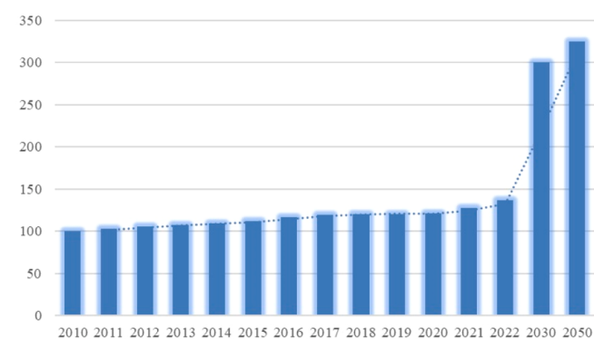
Fig. 13. Installed PHES and IRENA's global outlook (GW).
