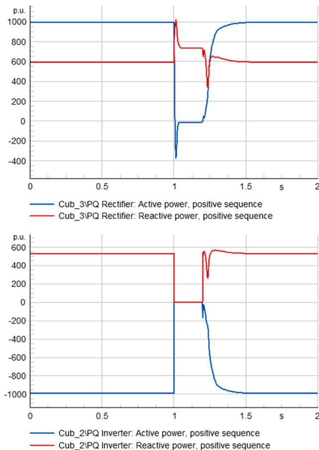
Fig. 21. Active and reactive power of the power electronic devices.
