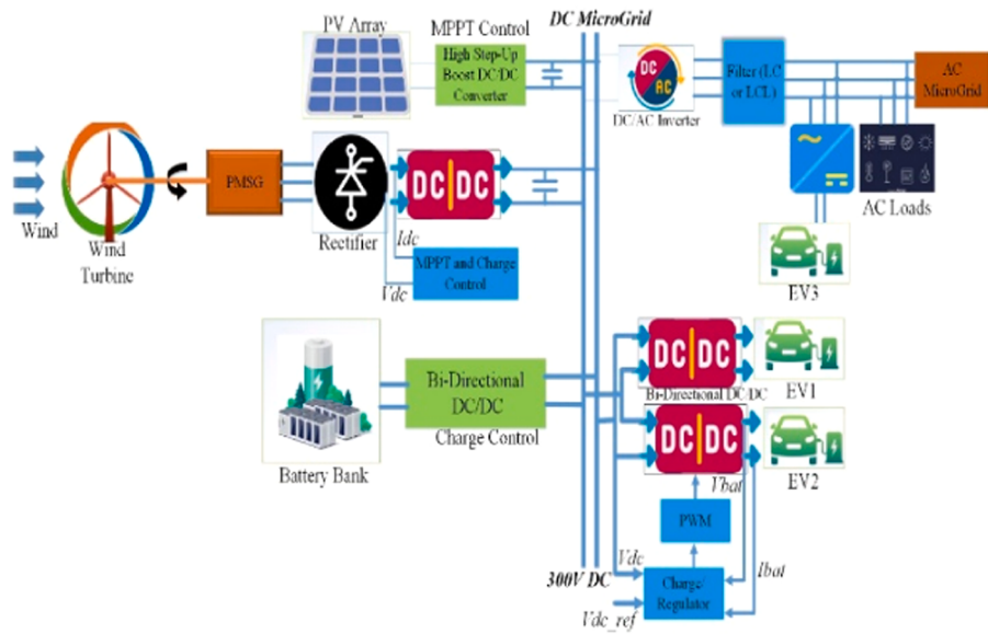
Fig. 18. DC and AC Microgrid.
