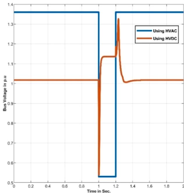
Fig. 20. Bus voltage using HVDC and HVAC.
