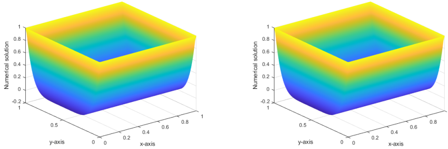
Figure 6: Left: h = 0.0078 , \min u_h = -2.5e-04 . Right: h = 0.0077 , \min u_h = +7.1e-14 .
