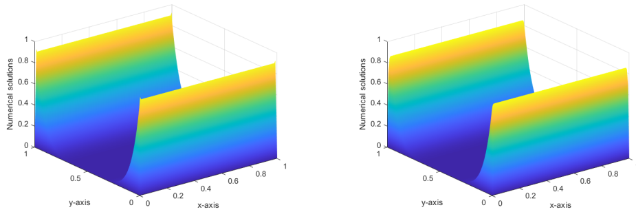
Figure 4: Left: h = 0.0075 , \min u_h = -8.8e - 14 . Right: h = 0.0074 , \min u_h = 0 .
