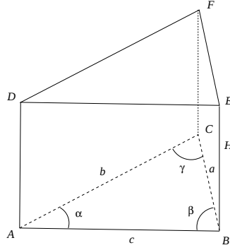
Figure 2: Basic notations for prismatic elements, based on [14].
