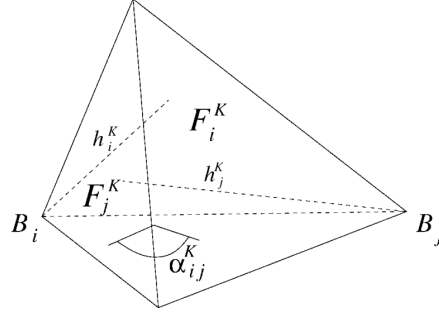
Figure 1: A tetrahedral cell K from [12].
