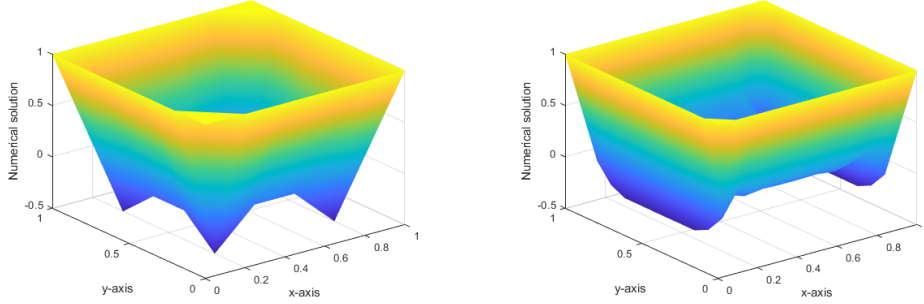
Figure 5: Left: h = 0.25 , \min u_h = -0.6157 . Right: h = 0.01 , \min u_h = -0.2689 .
