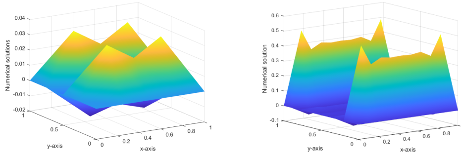
Figure 3: Left: h = 0.25 , \min u_h = -0.0170 . Right: h = 0.01 , \min u_h = -0.0421 .
