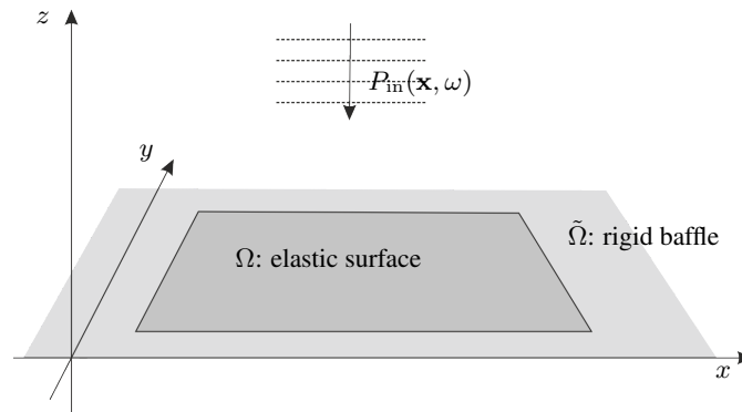
Figure 1. Geometry for scattering from an elastic surface.
