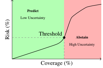
Figure 1: An example of selective classification where the task is to identify and categorize user complaints. Selective classification enables a model to assess uncertainty of each sample and abstain from predictions in situations when the prediction is deemed unreliable, allowing those cases to be handled by human reviewers.
