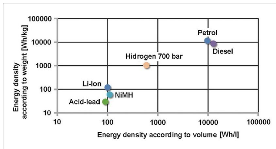
Figure 1: Tendencies of vehicle drive systems, 2010
