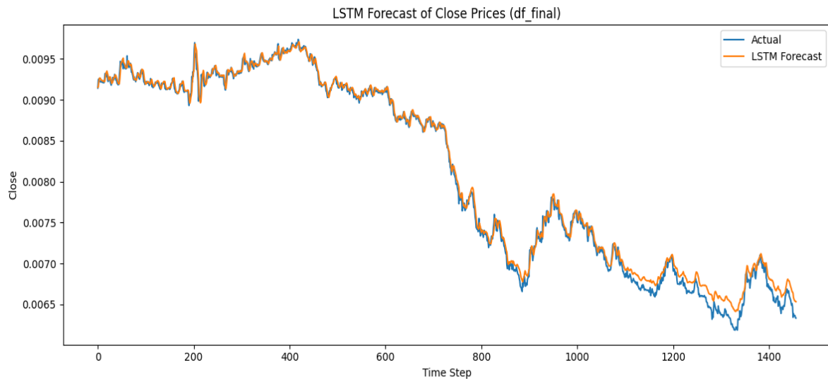
Figure 7: LSTM Model Performance
