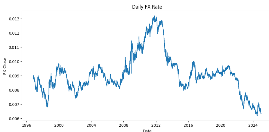
Figure 1: Yen Close price between 1996 and 2024
