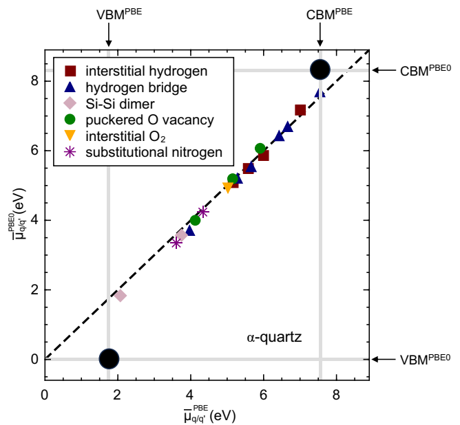
FIG. 1. Charge-state transition levels of various defects in \alpha -quartz calculated with the hybrid functional by Perdew, Ernzerhof, and Burke (commonly referred to as PBE0) 9 ( \bar{\mu}_{q/q'}^{\text{PBE0}} ) vs. corresponding levels calculated with the semilocal Perdew-Burke-Ernzerhof (PBE) functional 10 ( \bar{\mu}_{q/q'}^{\text{PBE}} ) upon alignment of the average electrostatic potential. The energy levels corresponding to the valence-band maximum (VBM) and the conduction-band minimum (CBM) as calculated with the two functionals are also shown (black disks). Reproduced with permission from Broqvist et al. , Phys. Status Solidi A 207 , 270 (2010). Copyright 2010 John Wiley and Sons.
