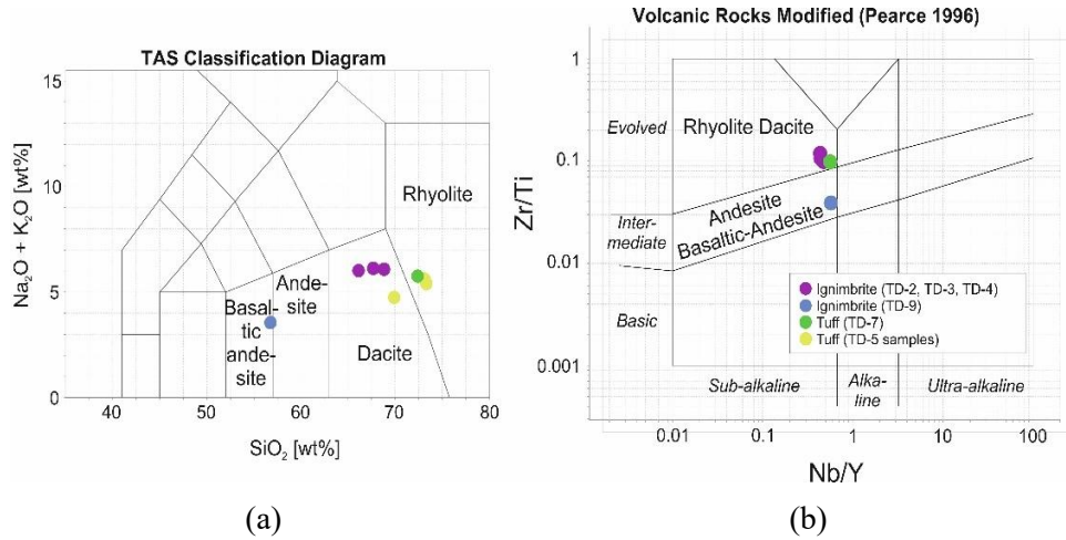
Figure 4 Rock classification plots for the studied samples. (a) TAS diagram, (b) Winchester-Floyd diagram
