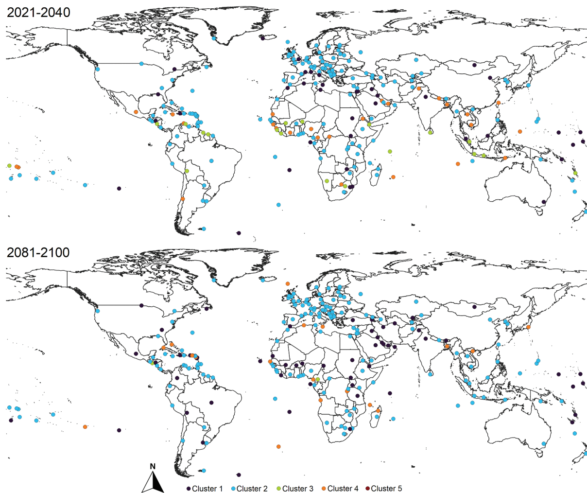
Figure 5. Distribution of dominant action activity clusters in the future periods 2021–2040 and 2081–2100.
