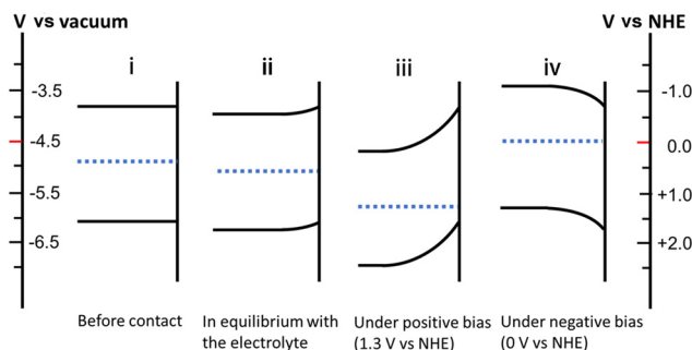
Fig. 3 Schematic band diagrams of (i) a bare BiFeO 3 electrode (ii) BiFeO 3 electrode in equilibrium with the electrolyte (iii) BiFeO 3 electrode under bias positive of the flat band potential (1.3 V vs. NHE) (iv) BiFeO 3 electrode under bias negative of the flat band potential (0 V vs. NHE). Before in contact with the electrolyte solution, there is no charge transfer thus no band bending (i). When the electrode comes into contact with the electrolyte solution, electrons transfer to the electrolyte to achieve equilibrium at which E_f of the electrode is the same as the redox potential of the electrolyte, which is 0.625 V vs. NHE. An upward band bending arises followed by the formation of the depletion region (ii). Under potentials positive to that of the flat band potential, E_f shifts more positively and the upward band bending increases (iii), producing anodic photocurrents. A depletion region can also be formed following downward band bending when potentials negative to that of the flat band potential are applied to the electrode, producing cathodic photocurrents.
