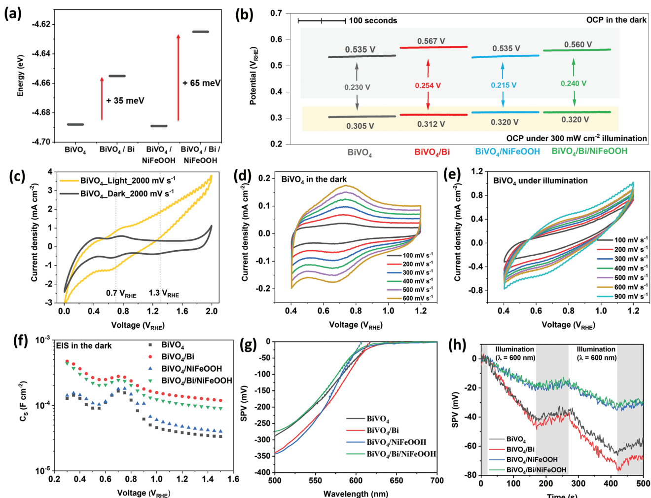
Figure 4. a) Fermi level of photoanodes measured by a vibrating tip Kelvin probe; b) OCP plots of photoanodes in the dark (grey background in graph) and under 300 mW cm -2 simulated sunlight (Xe source, AM 1.5G, yellow background in graph). 1000 mW cm -2 illumination results in the same values, but in an increase of noise and heating. c) CV plot of BiVO 4 at 2000 mV s -1 in the dark and under illumination. d) CV of BiVO 4 at various scan rates in the dark e) CV of BiVO 4 at various scan rates under illumination and corresponding linear relationship between peak current and (scan rate) 1/2 ; f) C s versus voltage obtained from fitting EIS data in the dark. The change of C s is related to the charge and discharge of surface states; g) Surface photovoltage of BiVO 4 photoanodes, showing an onset of the signal ≈600 nm. h) Negative SPV signal generated by two times repeated 100 s long sub-bandgap illumination (λ = 600 nm, indicated by white background color). All electrochemical measurements were done with N 2 purging to avoid any influence of ORR.
