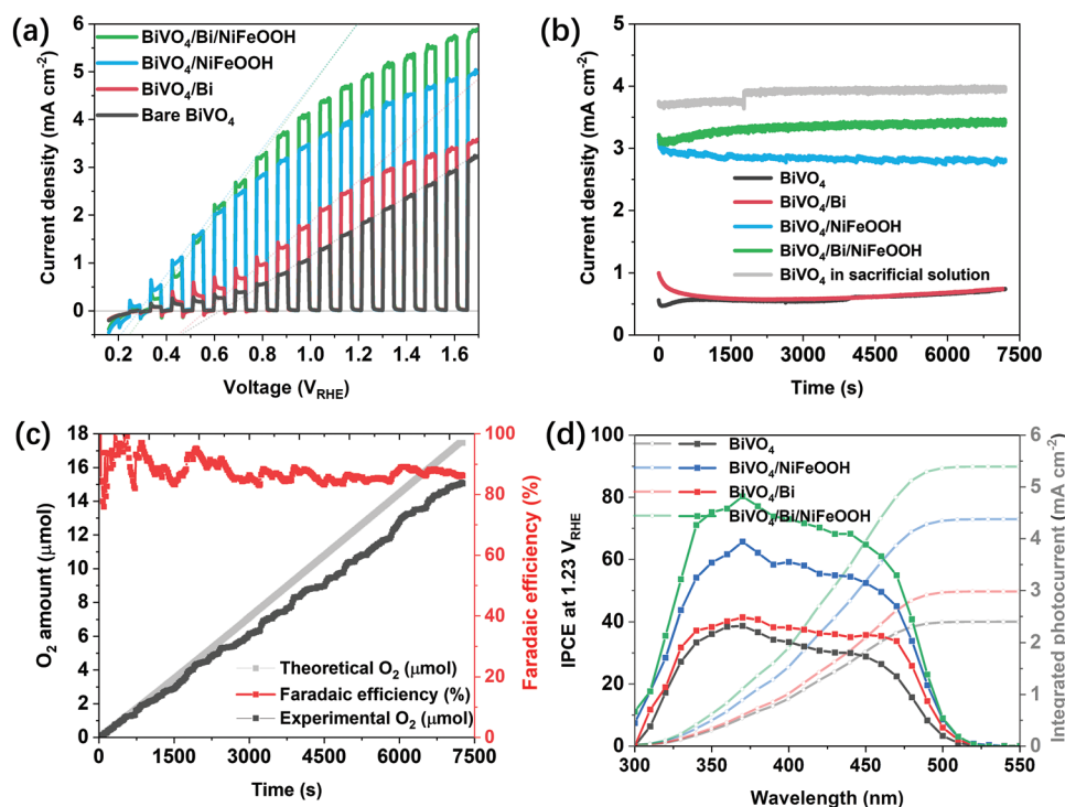
Figure 3. a) Photocurrent density-voltage curves of \text{BiVO}_4 photoanodes with chopped illumination. Voltage scan rate: 10 \text{ mV s}^{-1} . Reproducibility and error statistics are presented in Figure S11 (Supporting Information). b) Photocurrent density stability tests of photoanodes at +0.8 \text{ V}_{\text{RHE}} . c) Amount of measured and theoretical oxygen evolution and calculated faradaic efficiency at +0.8 \text{ V}_{\text{RHE}} . d) IPCE plots of \text{BiVO}_4 photoanodes at +1.23 \text{ V}_{\text{RHE}} (left) and integrated photocurrents (right). All these measurements were carried out in a 1 M KB buffer solution with pH 9 under simulated sunlight (Xe source, AM 1.5G filter, 100 \text{ mW cm}^{-2} ) or under monochromatic light (Xe source and monochromator). Measurement in (b) with sacrificial agent was carried out by adding 0.5 \text{ M Na}_2\text{SO}_3 to the same KB buffer solution.
