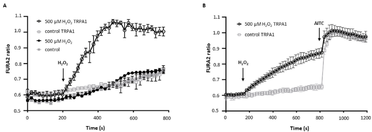
Fig. 8. \text{Ca}^{2+} measurements with Fura-2-AM in HEK293 cells expressing TRPA1. (A) TRPA1-dependent effect of \text{H}_2\text{O}_2 on [\text{Ca}^{2+}]_{\text{i}} . [\text{Ca}^{2+}]_{\text{i}} responses evoked by 500 \mu\text{M} \text{H}_2\text{O}_2 in the presence of TRPA1. (B) Change in [\text{Ca}^{2+}]_{\text{i}} of TRPA1 transfected HEK cells in response to sequential applications of 500 \mu\text{M} \text{H}_2\text{O}_2 and 10 \mu\text{M} AITC. Representative plot from at least 3 independent experiments shows the mean \pm SD of triplicate.
