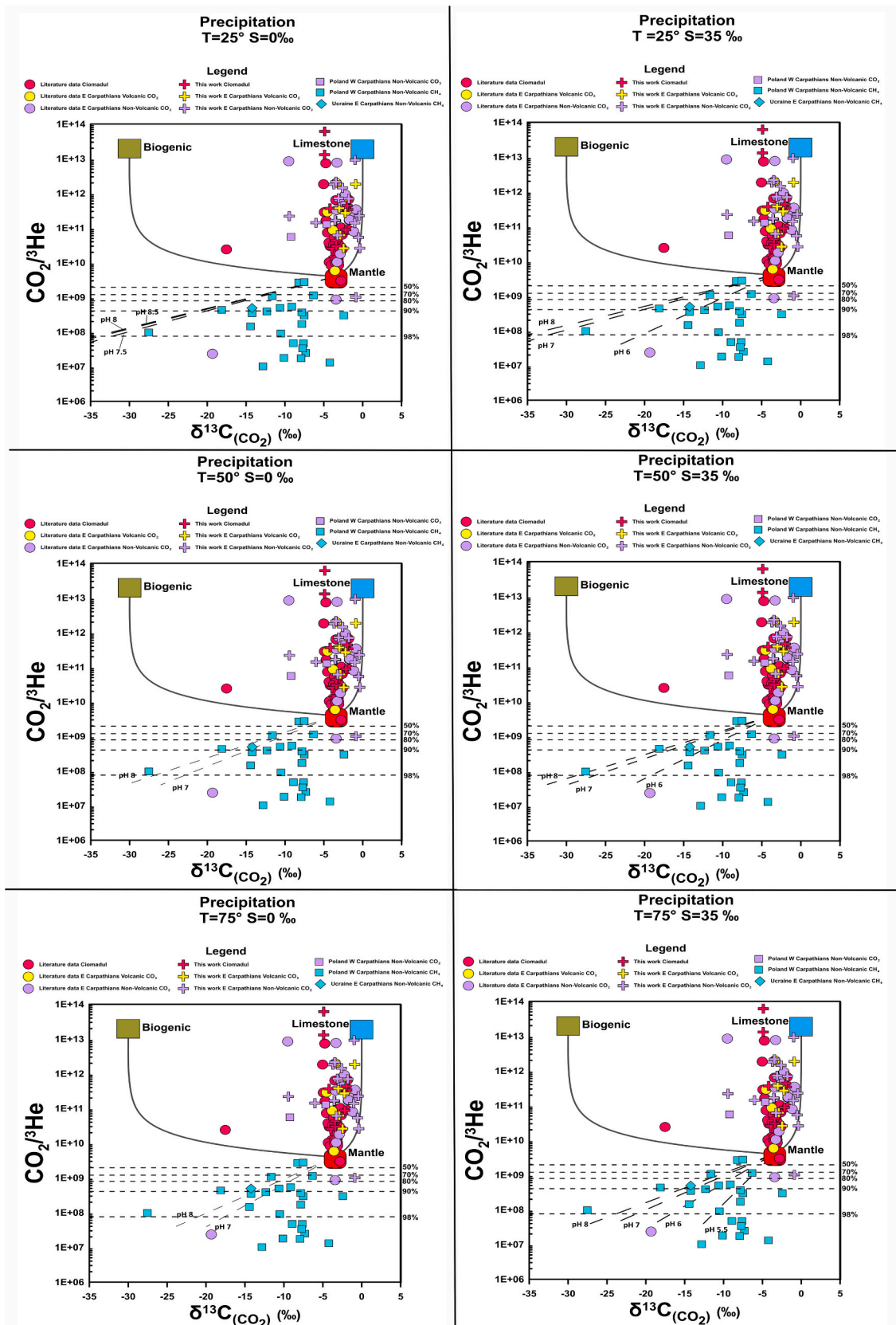
Fig. 11. \text{CO}_2/{}^3\text{He} vs. {}^{13}\text{C}\text{-CO}_2 of the investigated gas emissions. Lines show the theoretical mixing between a mantle end member (Bräuer et al., 2016; Rizzo et al., 2018) and crustal end members represented by marine limestones and organic sediments (Sano and Marty, 1995). Dashed lines represent the predicted trends for carbonate precipitation at different temperatures (25 °C, 50 °C and 75 °C) and salinity (S = 0‰ or S = 35‰), with the fractions of \text{CO}_2 removed from the fluid phase due to precipitation. Equations from Buttitia et al., (2023), Gilfillan et al. (2009) and Randazzo et al. (2025). Symbols as in Fig. 2.
