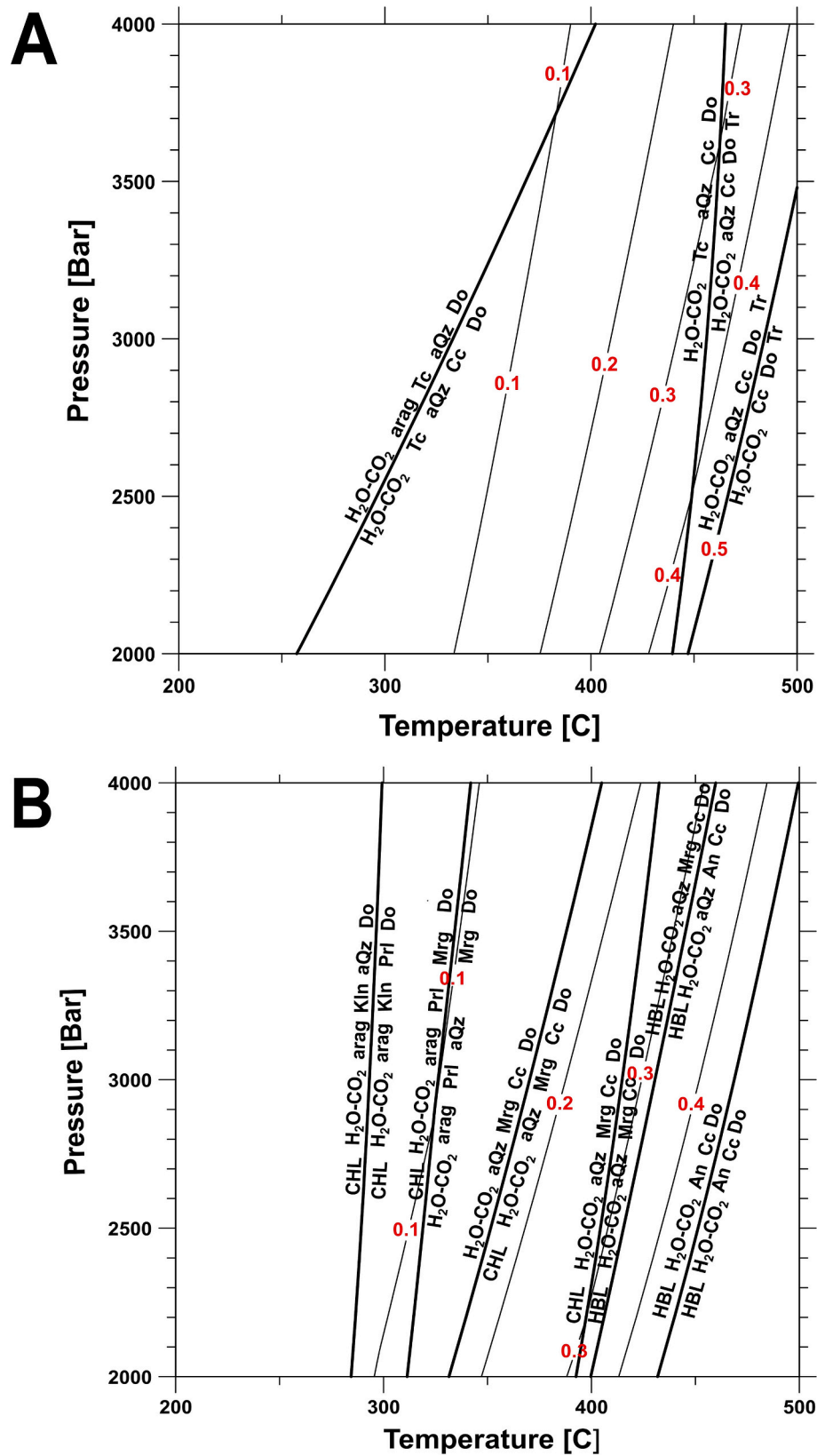
Fig. 8. Metamorphic processes generating CO 2 fluids computed by the Domino/Theriak code (De Capitani and Petrakakis, 2010) under physical conditions of P = 2000\text{--}4000 bar and T = 200\text{--}500 °C, with excess water. The thick lines in the figures of both models represent the primary reactions, while the thin lines show the partial pressure of the CO 2 in the CO 2 -H 2 O solution. Mineral abbreviations as follows: A. Cc-calcite, Do-dolomite, Tc-talc, arag-aragonite, aQz-alpha quartz, Tr-tremolite, B. Marl and kaolinite protolith Kln-kaolinite, Chl-chlorite, Prl-pyrophyllite, Mrg-margarite, Hbl-hornblende, An-anorthite minerals.
