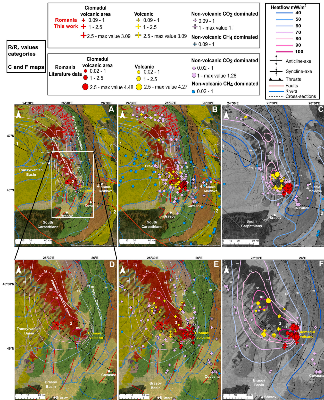
Fig. 6. Romanian segment of the Eastern Carpathians. A. Geology with heat flow data, references after Fig. 1 and (Horváth et al., 2006, 2015). B. Geology and chemical zoning of the gas emissions, references after Fig. 1. C. Non-contaminated ( ^4\text{He}/^{20}\text{Ne} > 1 ) He isotopic ratios vs. thermal heat flow. Zoomed versions: geology (D), chemical (E), non-contaminated ( ^4\text{He}/^{20}\text{Ne} > 1 ) He isotopic ratios vs. thermal heat flow (Horváth et al., 2006, 2015) (F). Symbols as in Fig. 1.
