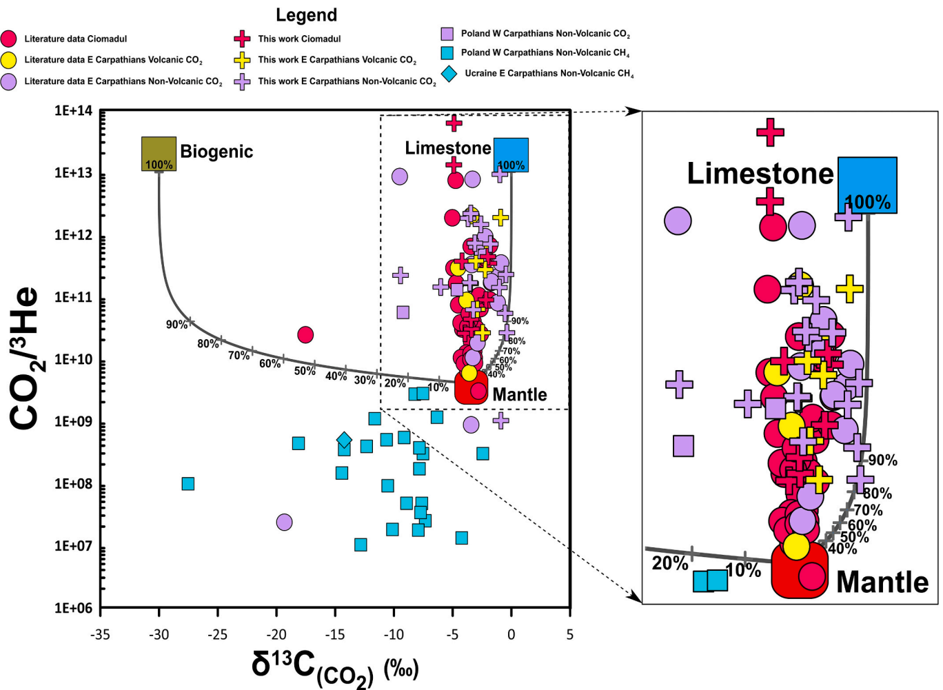
Fig. 9. \text{CO}_2/{}^3\text{He} vs. \delta^{13}\text{C}_{\text{CO}_2} plot of the investigated gas emissions. Lines show the theoretical binary mixing between a mantle end member ( \text{CO}_2/{}^3\text{He} = 2\text{--}7 \times 10^9 and \delta^{13}\text{C} = -3.5\text{‰} , Bräuer et al., 2016; Rizzo et al., 2018) and the crustal end members represented by marine limestones ( \text{CO}_2/{}^3\text{He} = 10^{13} , \delta^{13}\text{C} = 0\text{‰} ) and organic sediments ( \text{CO}_2/{}^3\text{He} = 1 \times 10^{13} , \delta^{13}\text{C} = -30\text{‰} ) (Sano and Marty, 1995). Curves labelled as 100–10% represent binary mixing trajectories between mantle and the crustal end-members, allowing the crustal and mantle contributions to be estimated directly from the position of each sample. Symbols as in Fig. 2.
