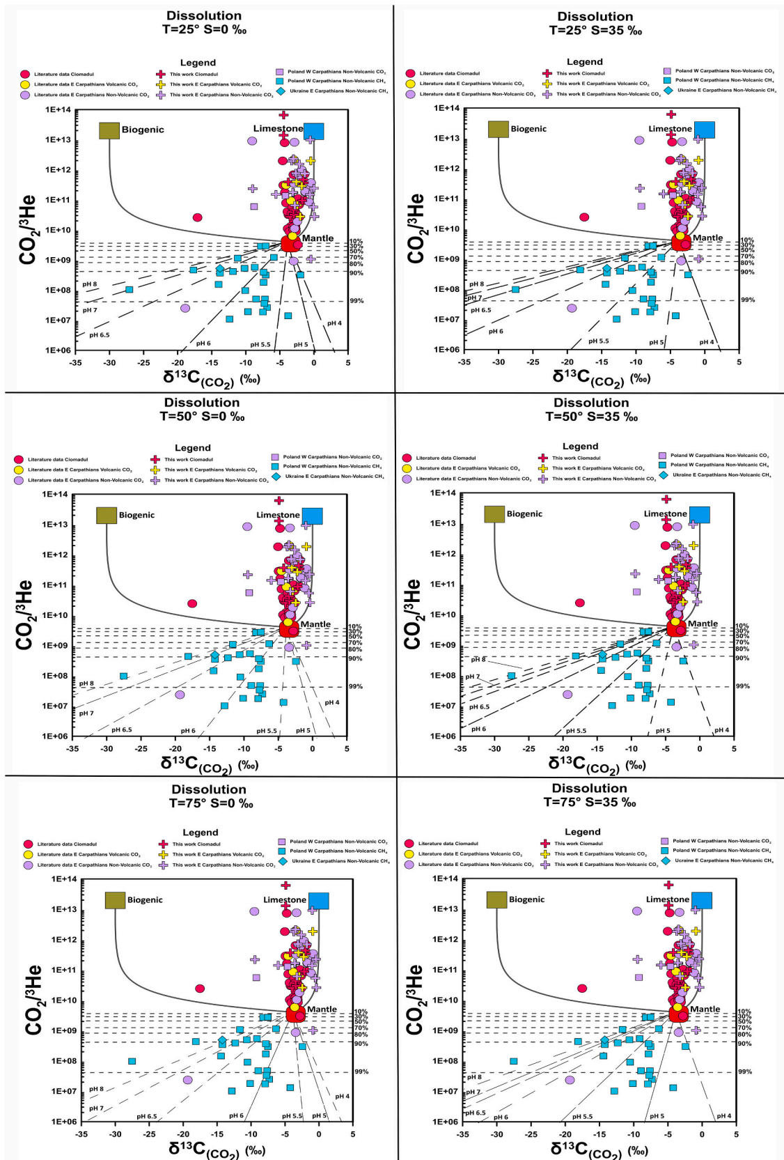
Fig. 10. \text{CO}_2/{}^3\text{He} vs. {}^{13}\text{C}\text{-CO}_2 of the investigated gas emissions. Lines show the theoretical binary mixing between a mantle end member (Bräuer et al., 2016; Rizzo et al., 2018) and crustal end members represented by marine limestones and organic sediments (Sano and Marty, 1995). Dashed lines represent the predicted model for a Rayleigh-type carbonate dissolution at different temperatures (25 °C, 50 °C and 75 °C) and salinity ( S = 0\text{‰} or S = 35\text{‰} ), with the fractions (%) of \text{CO}_2 lost from the gas phase due to dissolution into groundwater. Equations from Buttitta et al. (2023), Gilfillan et al. (2009) and Randazzo et al. (2025). Symbols as in Fig. 2.
