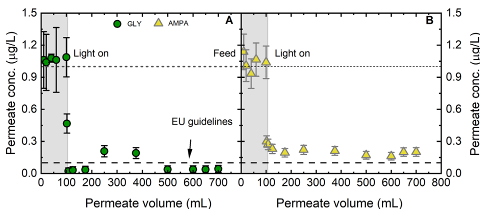
Figure 10. Permeate concentration of GLY (A) and AMPA (B) versus permeate volume at optimized conditions (PVDF- \text{TiO}_2 , c_f(\text{GLY}/\text{AMPA}) = 1 \mu\text{g L}^{-1} , J_w = 60 \text{ L m}^{-2} \text{ h}^{-1} , I(\text{AM}1.5 \text{ g } 350\text{--}1150 \text{ nm}) = 98 \text{ mW cm}^{-2} , \text{pH } 8.1 \pm 0.2 , 23 \pm 1^\circ \text{C} ).
