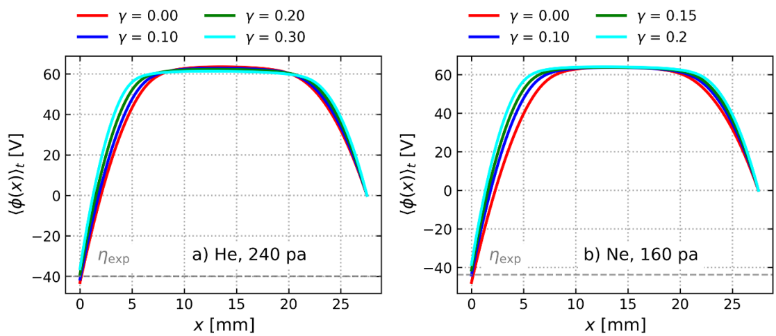
Figure 7. Spatial profiles of the time-averaged electrostatic potential \langle \phi(x) \rangle_t for (a) He at 240 Pa and (b) Ne at 160 Pa for different values of \gamma . The horizontal dashed line in each panel indicates the experimentally measured DC self-bias voltage \eta ( \eta = -40.0 V for He and \eta = -43.8 V for Ne). Discharge conditions: f_1 = 4 MHz, \phi_1 = 160 V, \phi_2 = 80 V, L = 2.75 cm, R = 0.7 , and \theta = 350^\circ .
