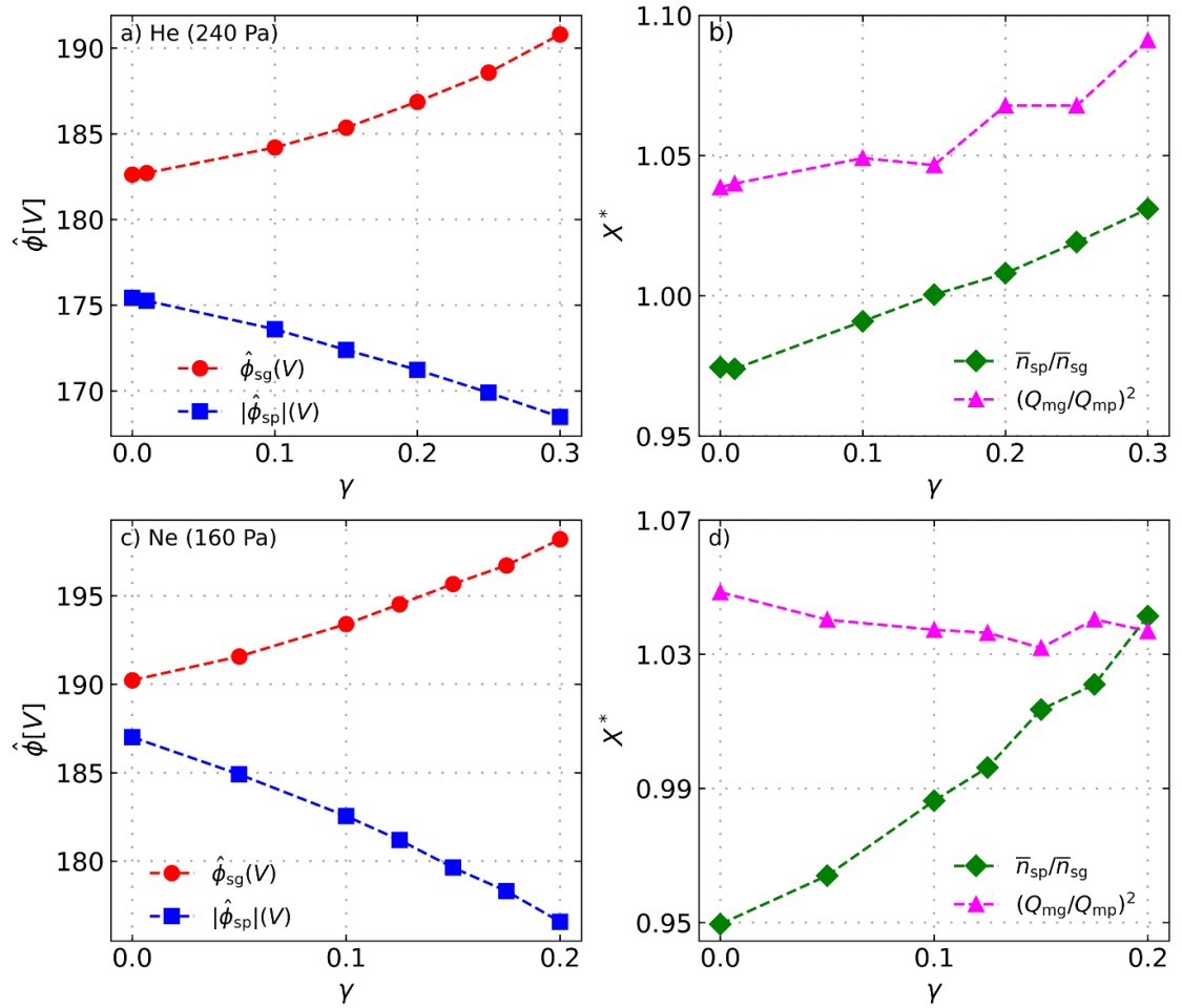
Figure 6. Peak sheath voltage values at the powered ( |\hat{\phi}_{sp}| ) and grounded ( \hat{\phi}_{sg} ) electrodes (a, c) and the ratios ( X^* ) of the mean charged particle densities in the respective sheaths, \bar{n}_{sp}/\bar{n}_{sg} , and the maximum uncompensated sheath charges, (Q_{mg}/Q_{mp})^2 , as functions of \gamma (b, d) for He (top row: p = 240 Pa) and Ne (bottom row: p = 160 Pa). Discharge conditions: L = 2.75 cm, f_1 = 4 MHz, \phi_1 = 160 V, \phi_2 = 80 V, R = 0.7 , at \theta = 350^\circ .
