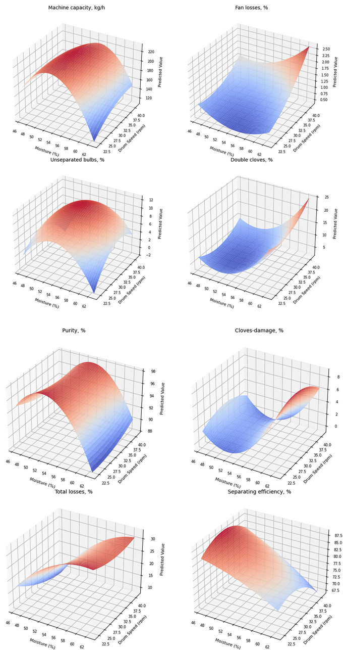
Fig. 5. Performance parameters at clearance = 10 mm. (Own source)
