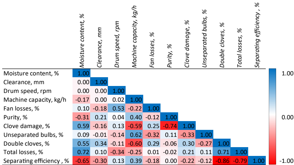
Fig. 4. The correlation matrix of key performance parameters of the developed garlic clove separation machine. (Own source)
