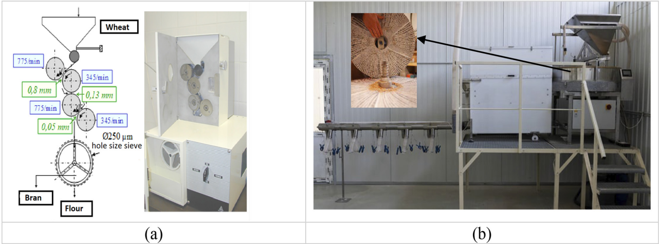
Fig. 1. Pictures of the lab mill (a) and Astrié mill (b) (Own source/creation)
