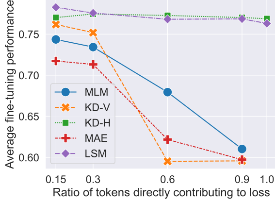
(a) Models after 10K pre-training steps
