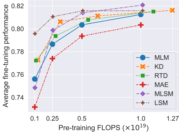
Figure 2: Overall fine-tuning scores obtained by differently pre-trained models at various pre-training stages. Markers indicate 10%, 25%, 50% and 100% pre-trained models. The location of the markers also reflects the different costs of the different pre-training objectives.
