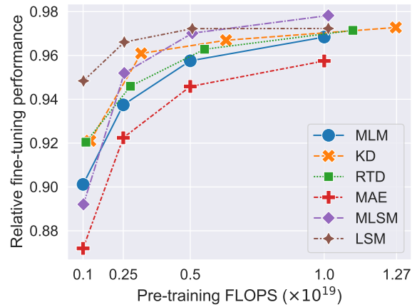
Figure 6: Relative performance of the differently trained PLMs compared to the fine-tuning results obtained by relying on the official ModernBERT model.
