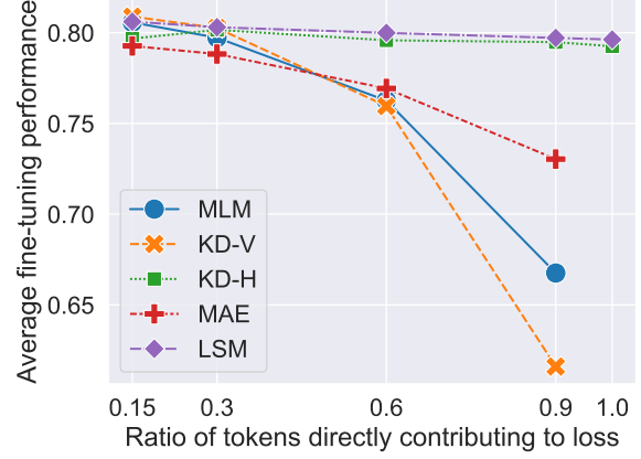
(b) Models after 100K pre-training steps
