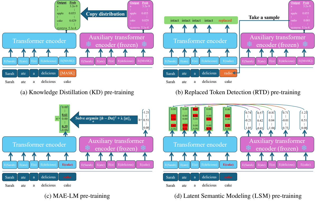
Figure 1: Overview of the different pre-training paradigms that rely on an auxiliary model. The auxiliary models are colored magenta, while the target outputs have a light green background. It is only the LSM pre-training (d) that is performed over the intact input sequence.
