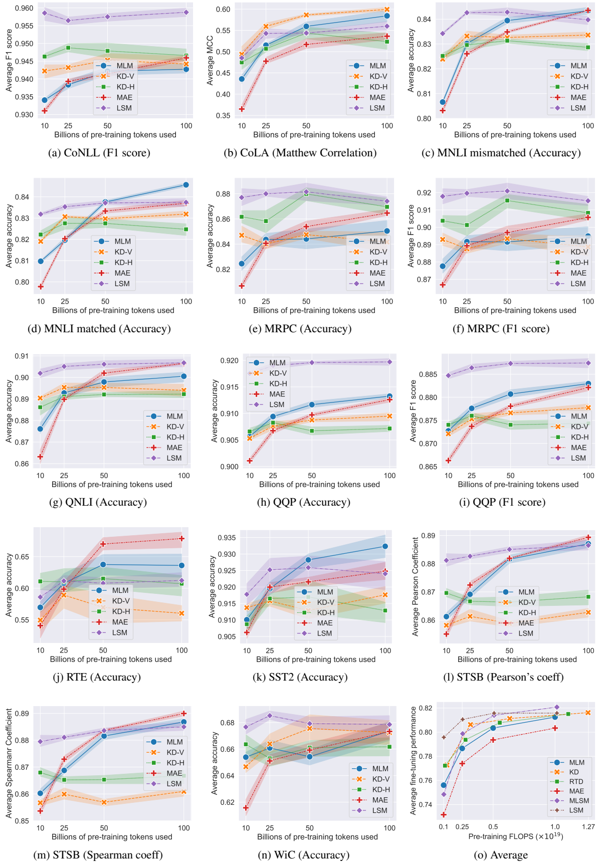
Figure 7: Fine-tuning results broken down for the individual evaluation metrics and differently pre-trained models at various readiness levels as indicated along the x-axis.
