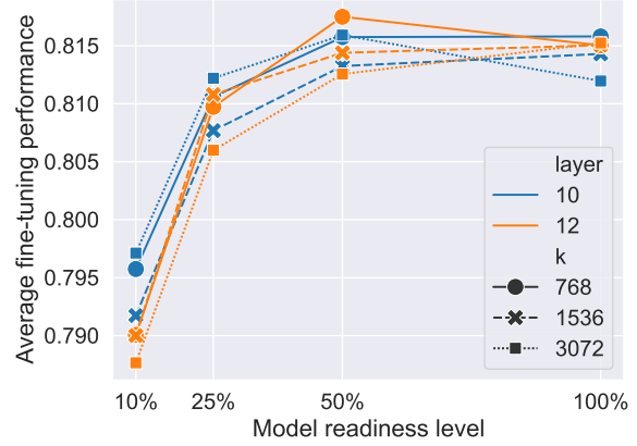
Figure 5: Comparing the fine-tuning performance of LSM models trained with different choices of l and k .
