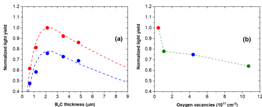
Figure 5. Normalized neutron irradiation-induced light yield of \text{Si/Ti}/(^{10}\text{B}_5\text{C}/\text{Ti})_n/\text{Al}_2\text{O}_3 layered substrate/absorber/scintillator structures as a function of (a) total ^{10}\text{B}_5\text{C} layer thickness; (b) areal density of oxygen vacancies in \text{Al}_2\text{O}_3 , for a fixed ^{10}\text{B}_5\text{C} thickness of 3.6\text{ }\mu\text{m} . In panel (a), dots show measured values while dashed lines indicate calculations. Red and blue colors represent two different oxygen vacancy contents in \text{Al}_2\text{O}_3 . In panel (b), the dashed line is only to guide the eye while the red and blue dots mark the \text{Al}_2\text{O}_3 scintillators used in the experiments shown in panel (a).
