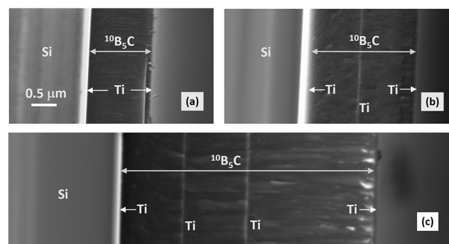
Figure 2. SEM cross-sectional micrographs of Si/Ti/ (^{10}\text{B}_5\text{C}/\text{Ti})_n structures with total ^{10}\text{B}_5\text{C} thickness of (a) 1.2 \mu\text{m} , (b) 2.35 \mu\text{m} , and (c) 4.8 \mu\text{m} . The thin Ti layers, located on top, below, or embedded in the \text{B}_5\text{C} films, are also indicated.
