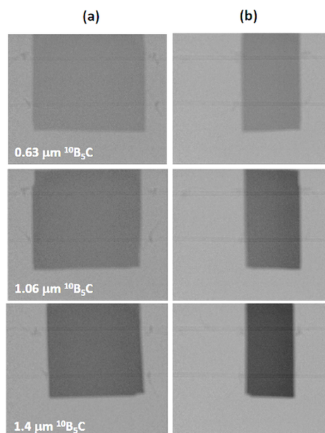
Figure 3. Neutron transmission images of isotopically enriched ^{10}\text{B}_5\text{C} layers with different thicknesses measured for sample tilt angles of (a) 0^\circ and (b) 60^\circ . The higher the neutron absorption, the darker the image of the absorber layer. Thin horizontal darker lines are the projected images of the Teflon strings.
