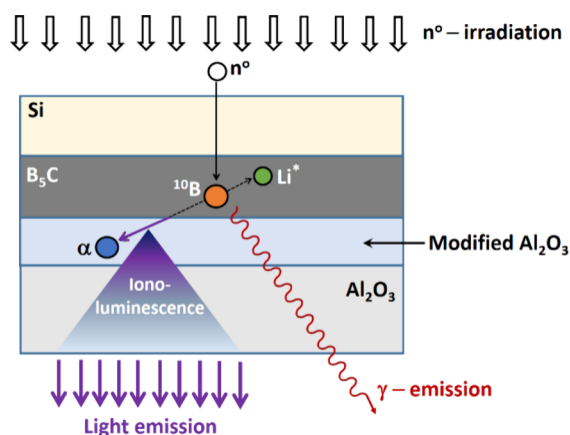
Figure 6. Schematic representation of neutron irradiation-induced ionoluminescence and \gamma -ray emission from a Si/ ^{10}\text{B}_5\text{C} /Al _2\text{O}_3 structure.
