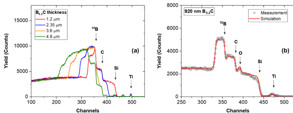
Figure 1. Sample 1.6 MeV p-EBS spectra of (a) Si/Ti/( 10 B 5.2 C/Ti) n structures with different total 10 B 5.2 C thicknesses and (b) Si/Ti/ 10 B 5.2 C-type sample with a 10 B 5.2 C thickness of 920 nm together with its RBX simulation. Spectrum edges for Ti, Si, O, C, and 10 B are indicated by arrows. For more details, see the text.
