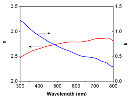
Figure 7. Pseudo n and k spectra of a sputter-deposited amorphous ^{10}\text{B}_5\text{C} layer evaluated from spectroscopic ellipsometry measurements.
