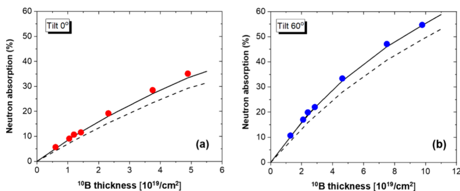
Figure 4. Neutron absorption as a function of effective ^{10}\text{B} thickness for isotopically enriched ^{10}\text{B}_5\text{C} layers deposited on the Si substrate, measured at (a) 0^\circ and (b) 60^\circ sample tilt angles with respect to the neutron beam. Symbols: measurement, dashed line: calculation considering the ^{10}\text{B}_5\text{C} absorption effect only, solid line: calculation considering ^{10}\text{B}_5\text{C} -related neutron absorption, Si substrate-related neutron attenuation, and neutron absorption/conversion in the ^6\text{LiF/ZnS:Cu} scintillation screen. Neutron energy dependence for these processes was also considered.
