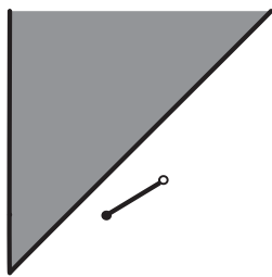
Figure 1: The domain \tilde{\Omega}_2 .
