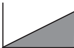
Figure 2: The domain \tilde{\Omega}_1 .
