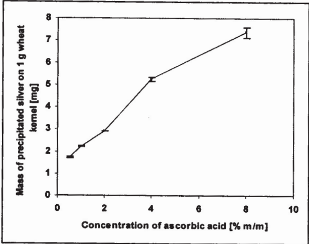
Figure 5. Effect of ascorbic acid on the mass of the precipitated silver on 1 g wheat kernel sample. The silver-amine concentration was 0.1 M.
