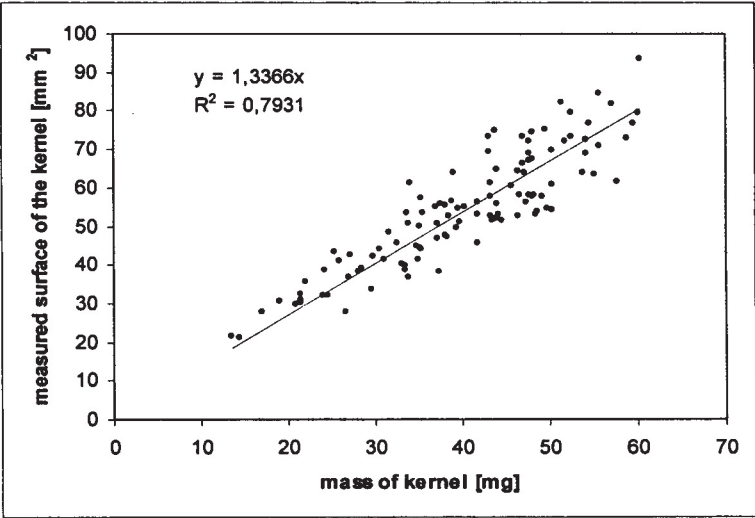
Figure 7. The measured surface area versus mass of kernel in case of MV 21 wheat variety.
