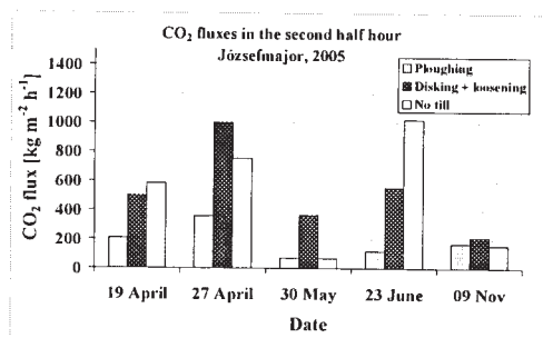
Figure 3. CO 2 fluxes in the second half hour (Józsefmajor, 2005)
