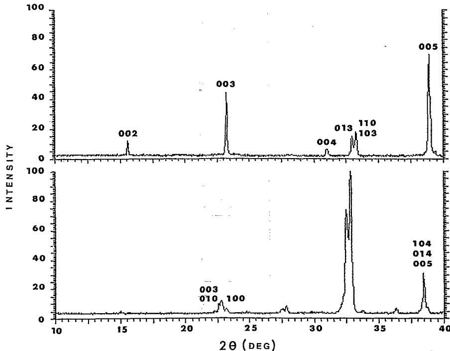
FIG. 1. Part of the diffraction pattern sample C (upper curve) compared with a nearly random powdered sample (lower curve) of \text{YBa}_2\text{Cu}_3\text{O}_{7-\delta} . The (00 l ) reflections are stronger in the bulk sample indicating a substantial orientation of the surface grains. The upper curve is displaced slightly to higher angles due to the placement of the pellet surface relative to the center of the goniometer.
