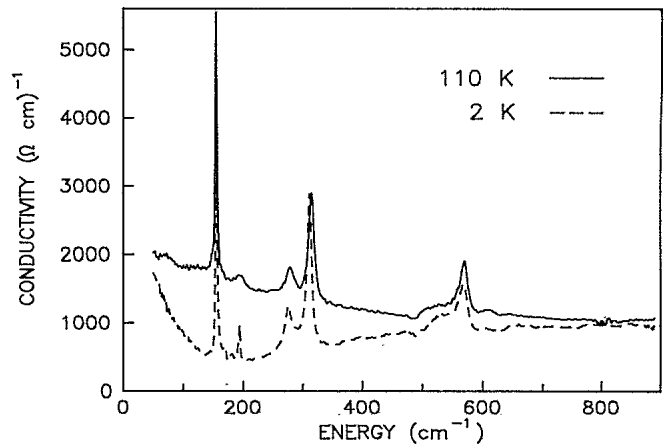
FIG. 4. Real part of the conductivity of \text{YBa}_2\text{Cu}_3\text{O}_{7-s} in the normal state (solid curve) and in the superconducting state (dashed curve) from Kramers-Kronig analysis of the reflectance of sample C (unpolished and freshly annealed in oxygen). We consider the suppression of low far-infrared conductivity at the superconducting transition and the narrowing of low-lying phonon lines evidence for the existence of an energy gap.
