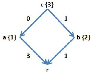
Figure 3: The supermodularity of the characteristic function
