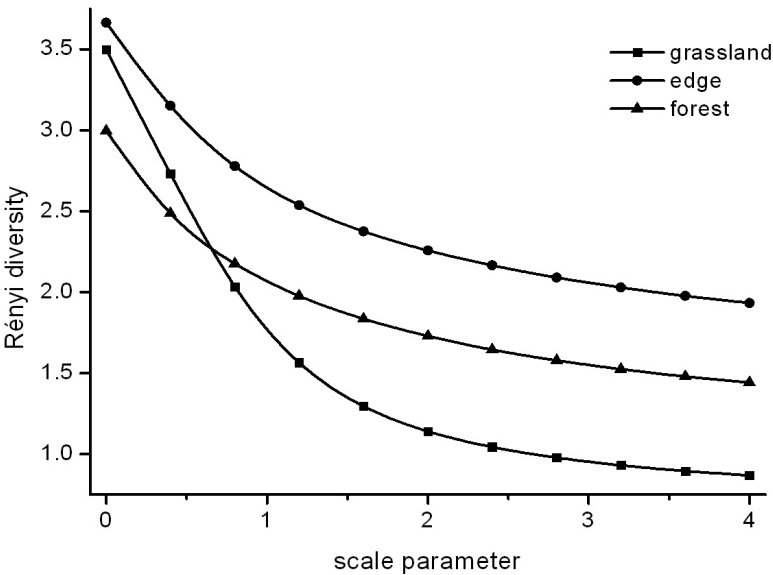
Figure 2. Diversity profiles of the carabid assemblages of the studied habitats.
