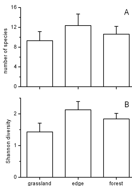
Figure 1. Number of species (A) and the Shannon diversity (B) of carabids per trap (with S.D.) in the studied habitats.
