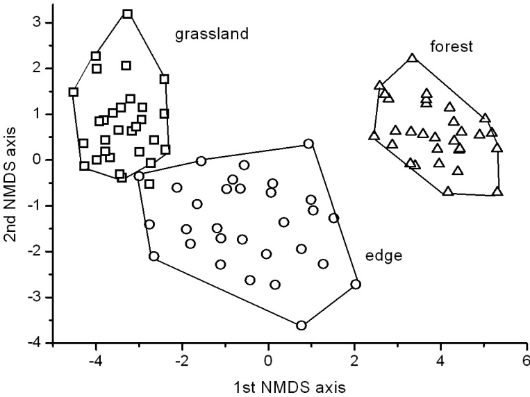
Figure 3. Ordination (NMDS) of the pitfall catches based on the abundance of the species after a logarithmic transformation using the Euclidean distance of the logarithmically transformed counts.
