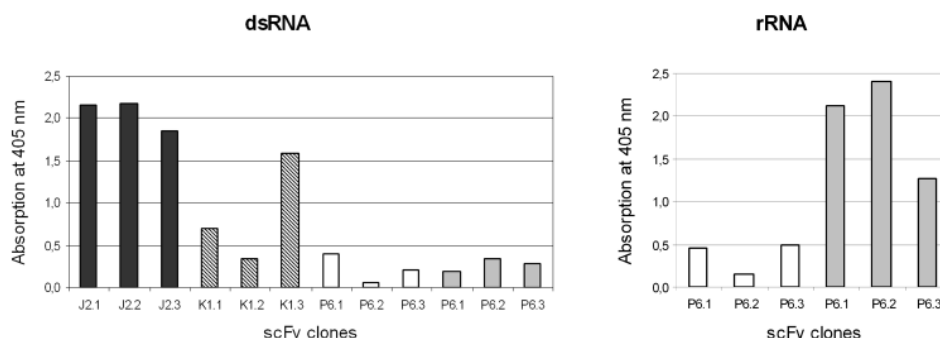
Fig. 1. Antigen binding activity of bacterially expressed J2-, K1- and P6-scFvs in ELISA. scFv from periplasmic extracts of different transformed colonies were immobilised by anti-E-tag monoclonal antibodies on ELISA plates. Biotinylated dsRNA or ribosomal RNA at 15 ng/well was used as antigen. The figure shows that J2- and K1-scFvs retained their dsRNA-binding activity, while P6-scFvs have a much higher affinity to rRNA than to dsRNA
