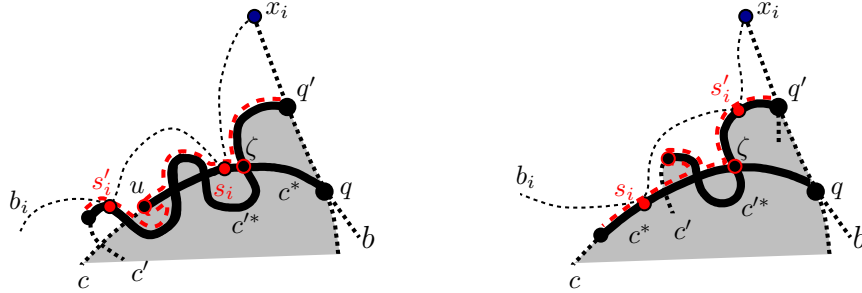
Figure 10: Constructing the curve W – the two intersecting scenarios. Notice that the first intersection \zeta of c^* with c must belong to c^* . Left: In the first intersecting scenario, W may have to retrace the last segment of U . Notice that c' \cap W consists only of segments of c^* (while c can meet W at a point outside c^* ). Right: In the second intersecting case, W may have to retrace the last segment of U' , and c \cap W consists only of segments of c^* .
