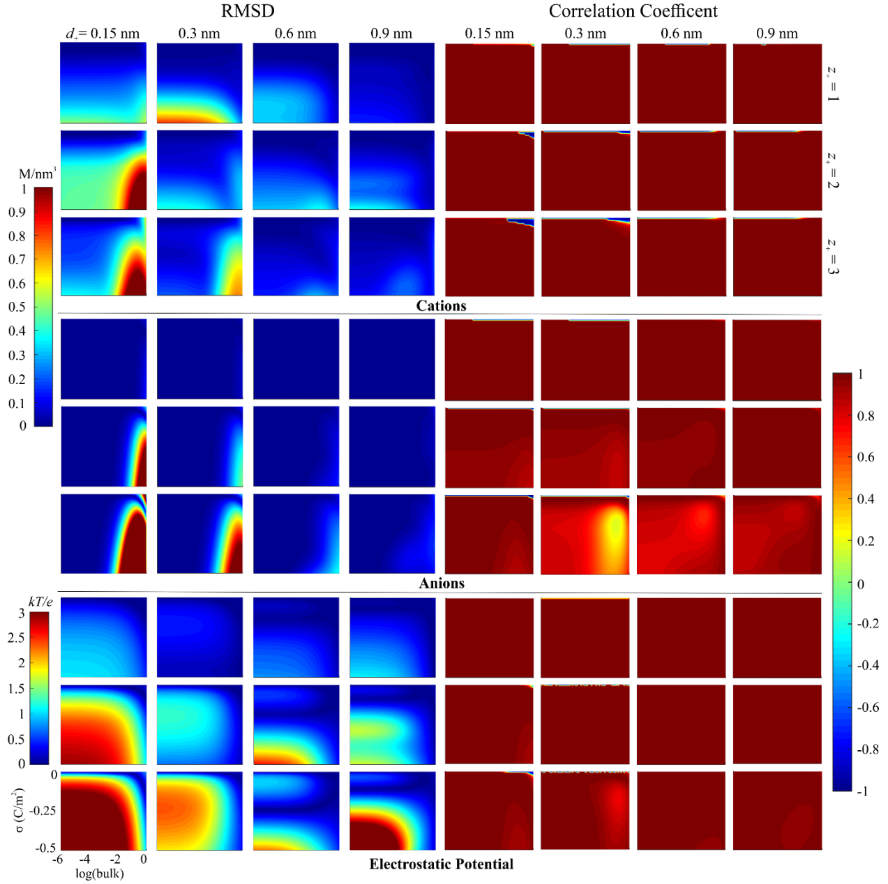
Fig. A1. Plots comparing the RMSD (left) and the Pearson correlation coefficients (right) for the RFD and BF functionals: \rho_+(x) (top), \rho_-(x) (middle), and \phi(x) (bottom). The logarithm of \rho_+^{\text{bulk}} is shown on the x -axis and \sigma is shown on the y -axis of each individual plot. Each row of plots corresponds to z_+ and the columns to d_+ as indicated. The group numbers of areas of difference are shown near the corresponding areas with significant deviation. The maximum values for the RMSD scales are 4.17 M (cations and anions) and 5.17 kT/e (electrostatic potential); this results in oversaturation for some of the plots. The same scales as in Fig. 1 of the main text are used.
