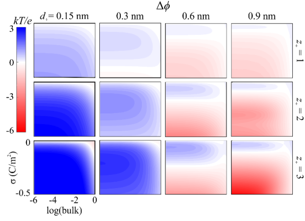
Fig. A5. Plots comparing \Delta\phi for the RFD and BF functionals at the charged surface. The plot axes and arrangements are as in Figure 1 Supplementary.
