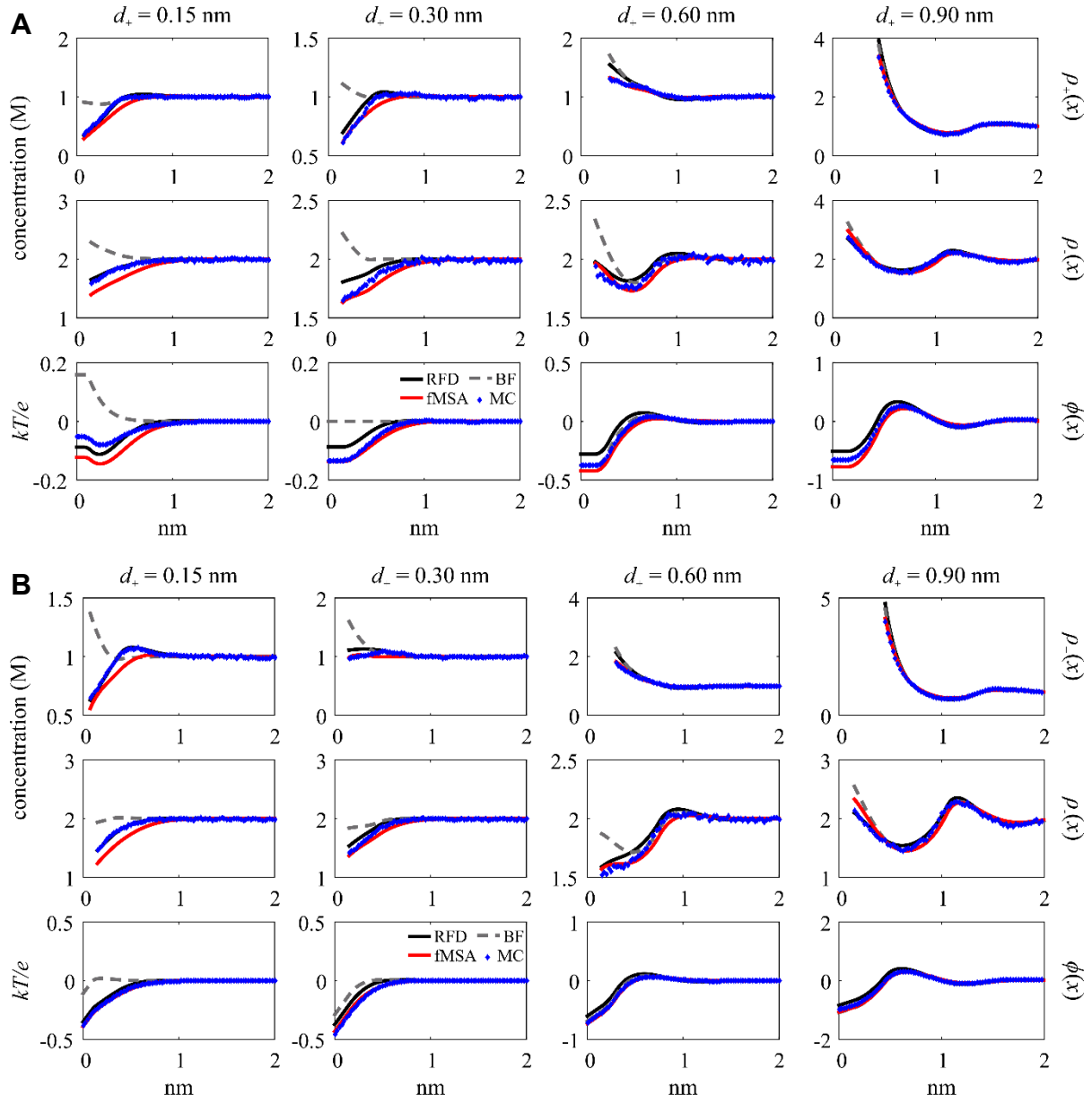
Fig. A3. DFT and MC \rho_+(x) , \rho_-(x) , and \phi(x) (labeled at right) plotted for \rho_+^{\text{bulk}} = 1 M and \sigma = 0 C/m 2 (A) and -0.02 C/m 2 (B) for all divalent ions across all diameters (labeled at top).
