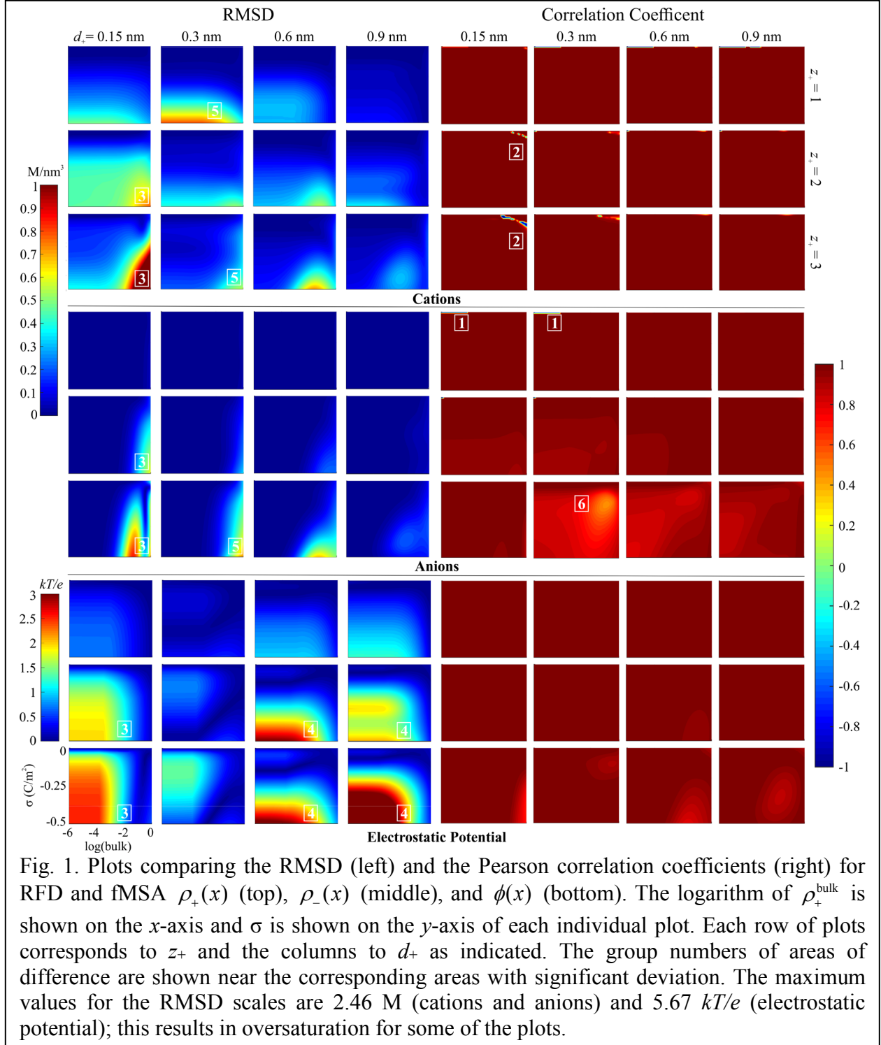
Fig. 1. Plots comparing the RMSD (left) and the Pearson correlation coefficients (right) for RFD and fMSA \rho_+(x) (top), \rho_-(x) (middle), and \phi(x) (bottom). The logarithm of \rho_+^{\text{bulk}} is shown on the x-axis and \sigma is shown on the y-axis of each individual plot. Each row of plots corresponds to z_+ and the columns to d_+ as indicated. The group numbers of areas of difference are shown near the corresponding areas with significant deviation. The maximum values for the RMSD scales are 2.46 M (cations and anions) and 5.67 kT/e (electrostatic potential); this results in oversaturation for some of the plots.
