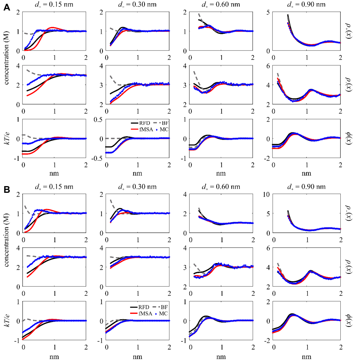
Fig. A4. DFT and MC \rho_+(x) , \rho_-(x) , and \phi(x) (labeled at right) plotted for \rho_+^{\text{bulk}} = 1 \text{ M} and \sigma = 0 \text{ C/m}^2 (A) and -0.02 \text{ C/m}^2 (B) for all trivalent ions across all diameters (labeled at top).
