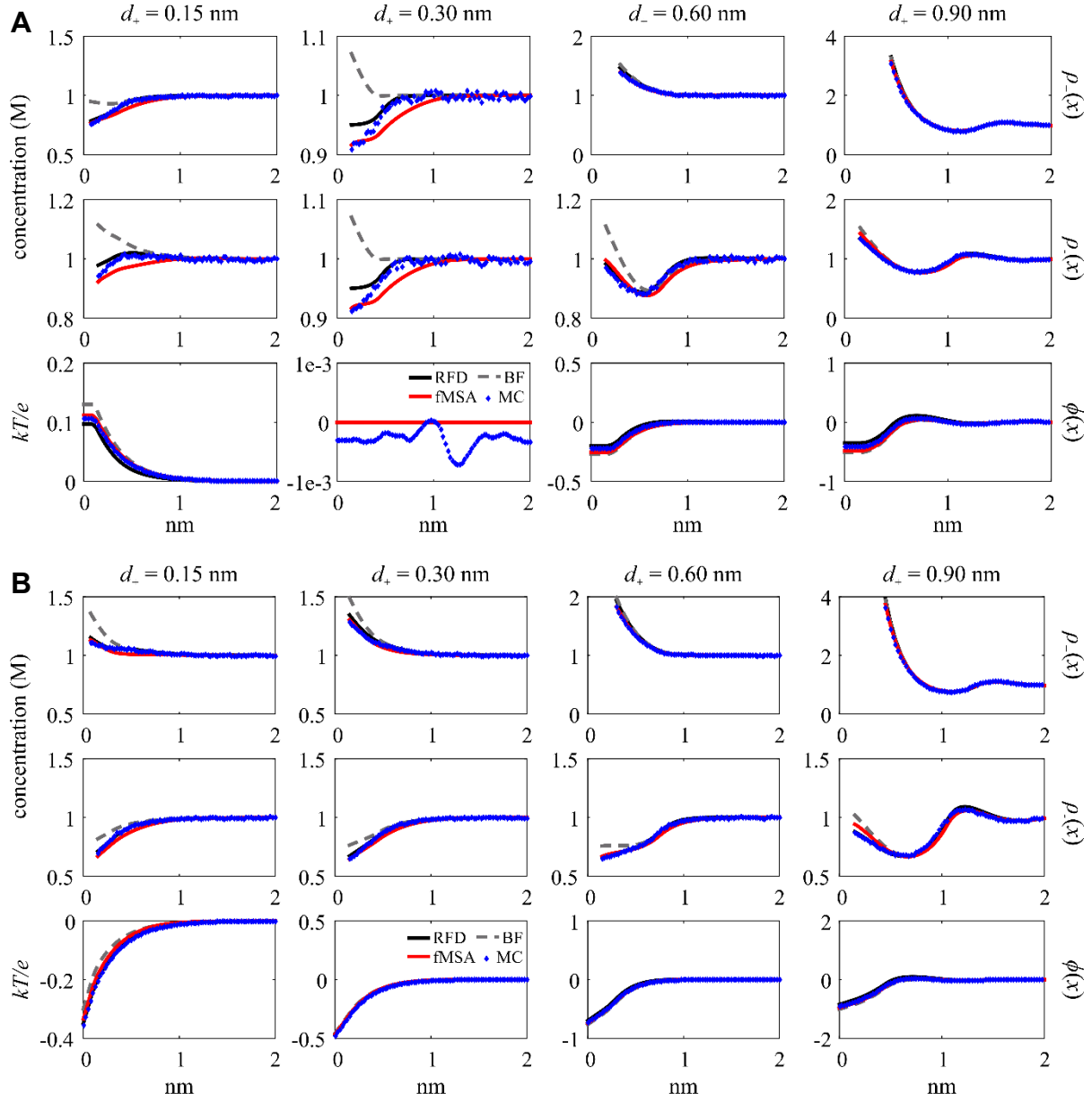
Fig. A2. DFT and MC \rho_+(x) , \rho_-(x) , and \phi(x) (labeled at right) plotted for \rho_+^{\text{bulk}} = 1 \text{ M} and \sigma = 0 \text{ C/m}^2 (A) and -0.02 \text{ C/m}^2 (B) for all monovalent ions across all diameters (labeled at top).
